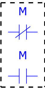
Contactor Aux Contacts
