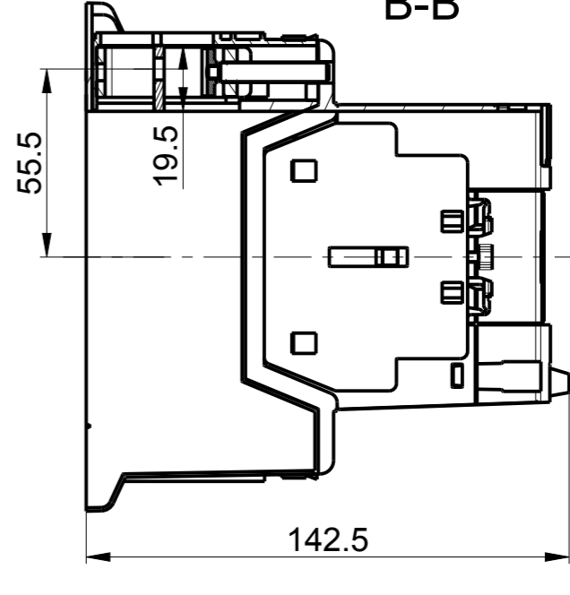
ASM, 100-E116E*/-E146E*, 300-EOE* CAD MODEL 10003595331
