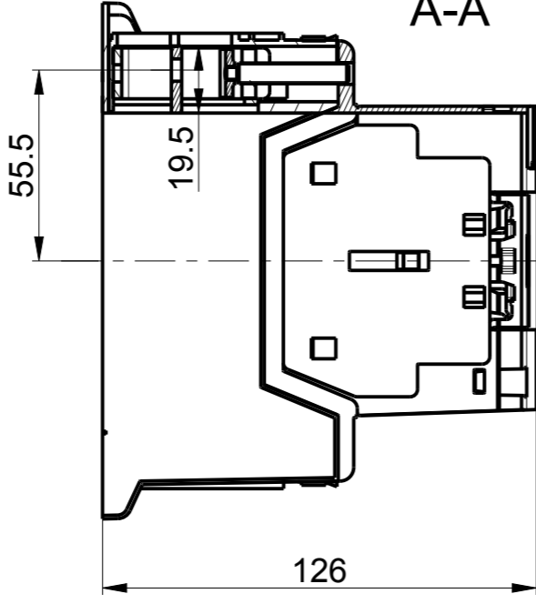
ASM, 100-E116*/-E146*, 300-EO* CAD MODEL 10002701129
