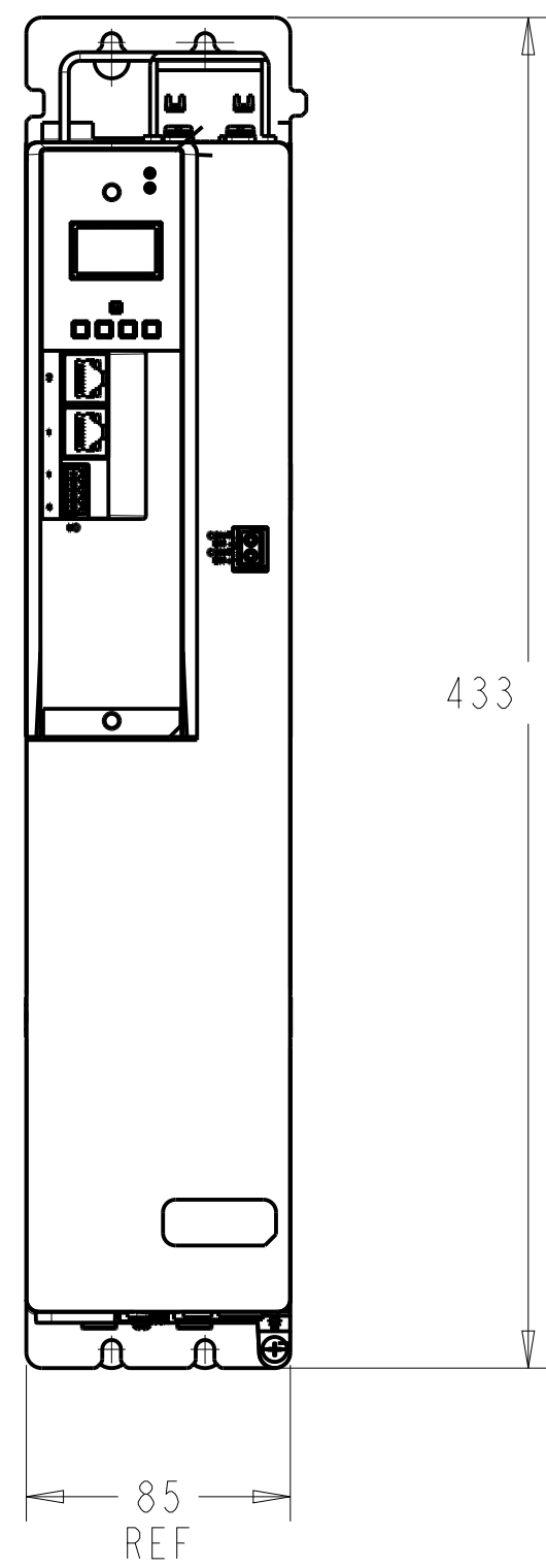
FRONT VIEW
