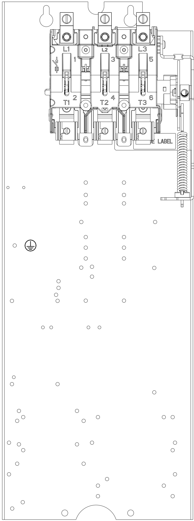
PANEL LAYOUT (FRONT)
