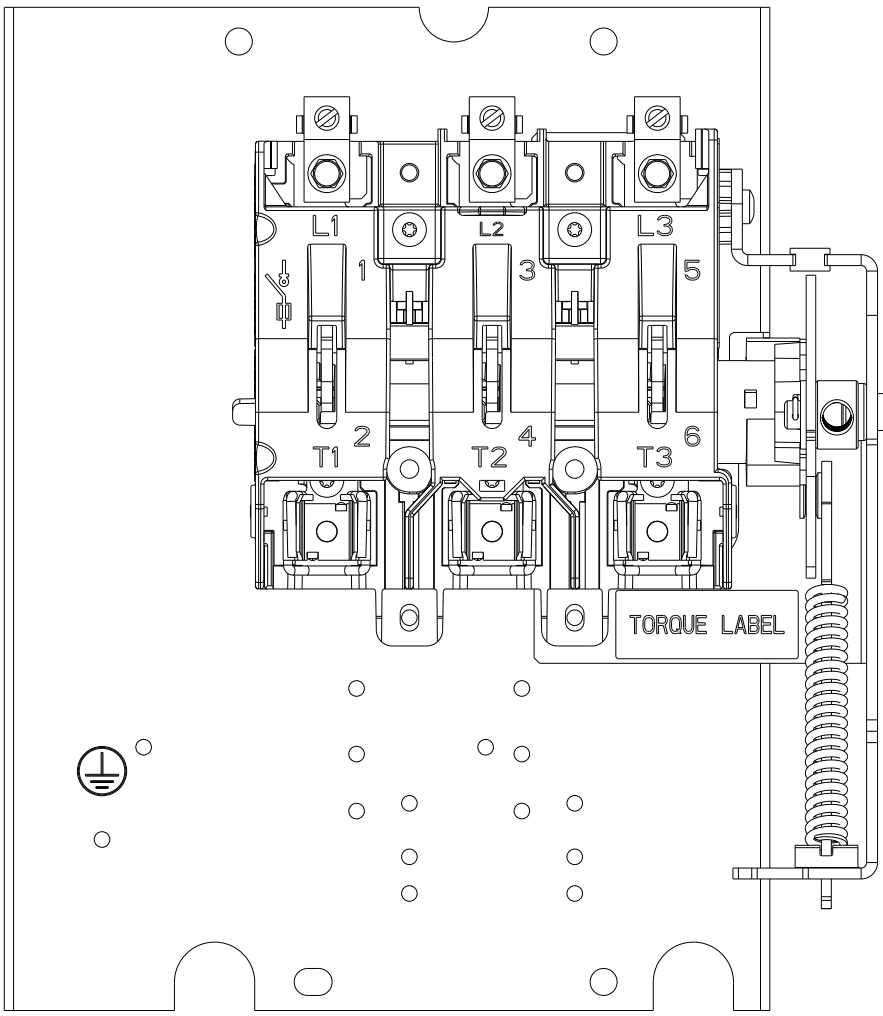
PANEL LAYOUT (FRONT) J FUSE LOCATION SHOWN
