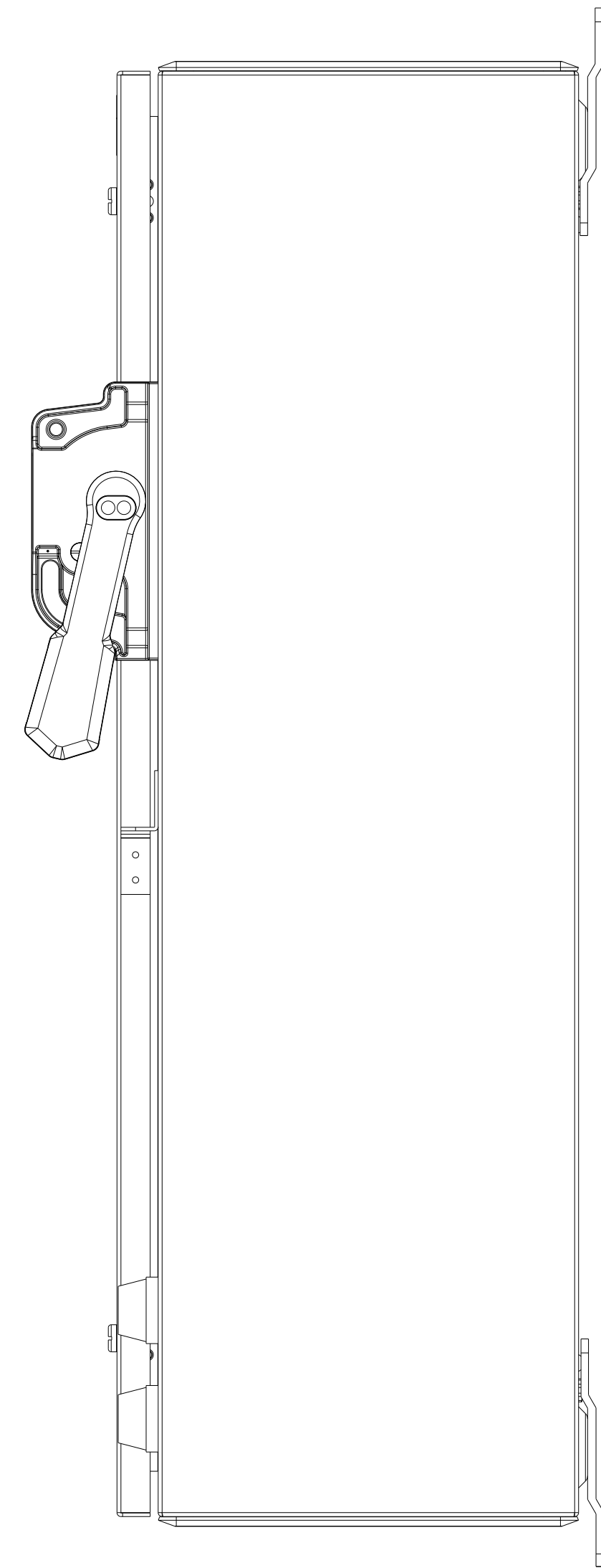
PANEL LAYOUT (SIDE) ENCLOSURE SHOWN W/DOOR, THIS VIEW
