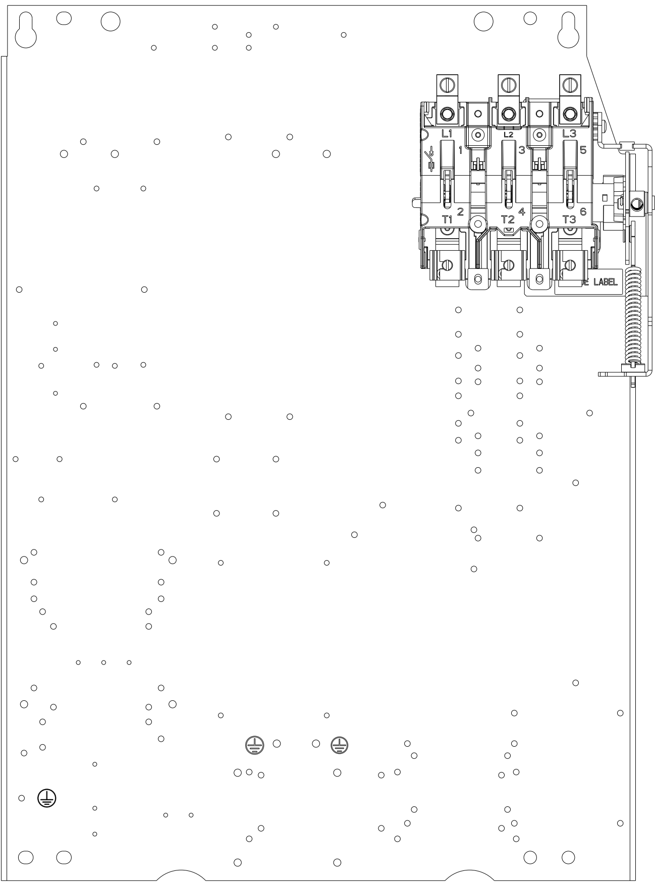
PANEL LAYOUT (FRONT)
