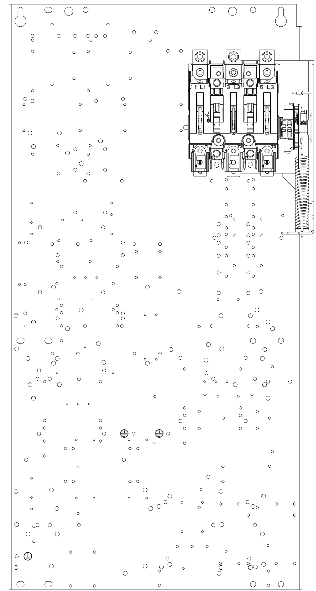
PANEL LAYOUT (FRONT)
