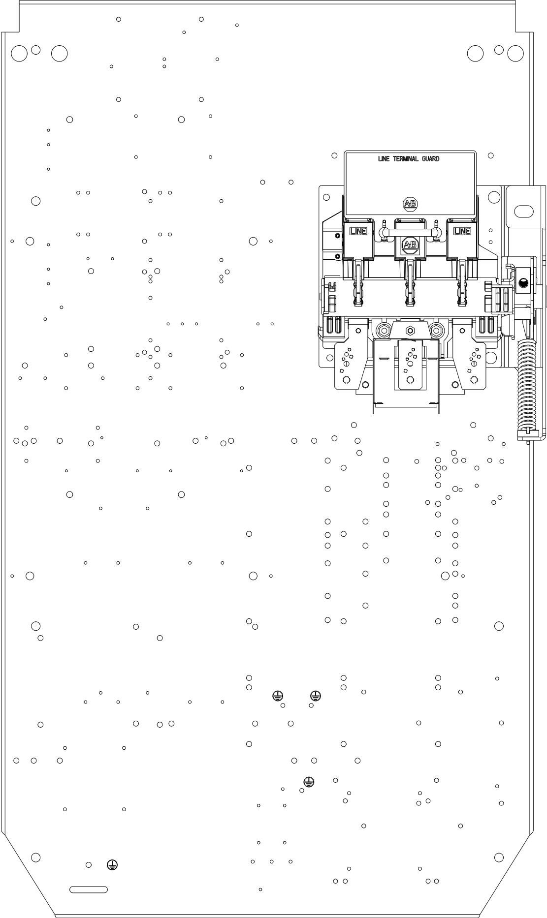
PANEL LAYOUT (FRONT)
