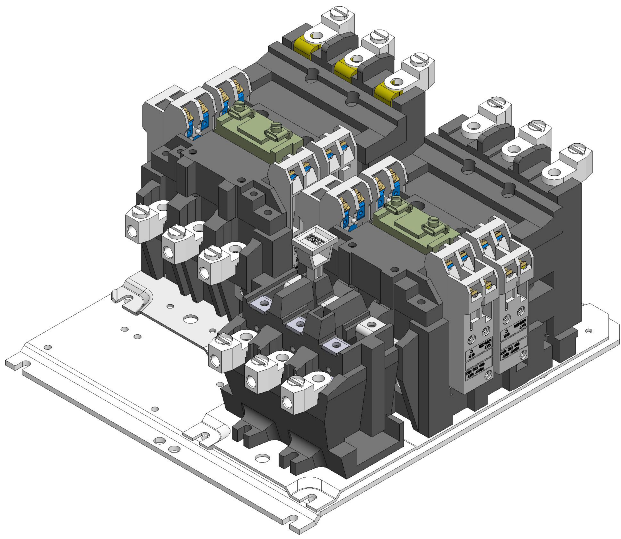
ISOMETRIC VIEW
