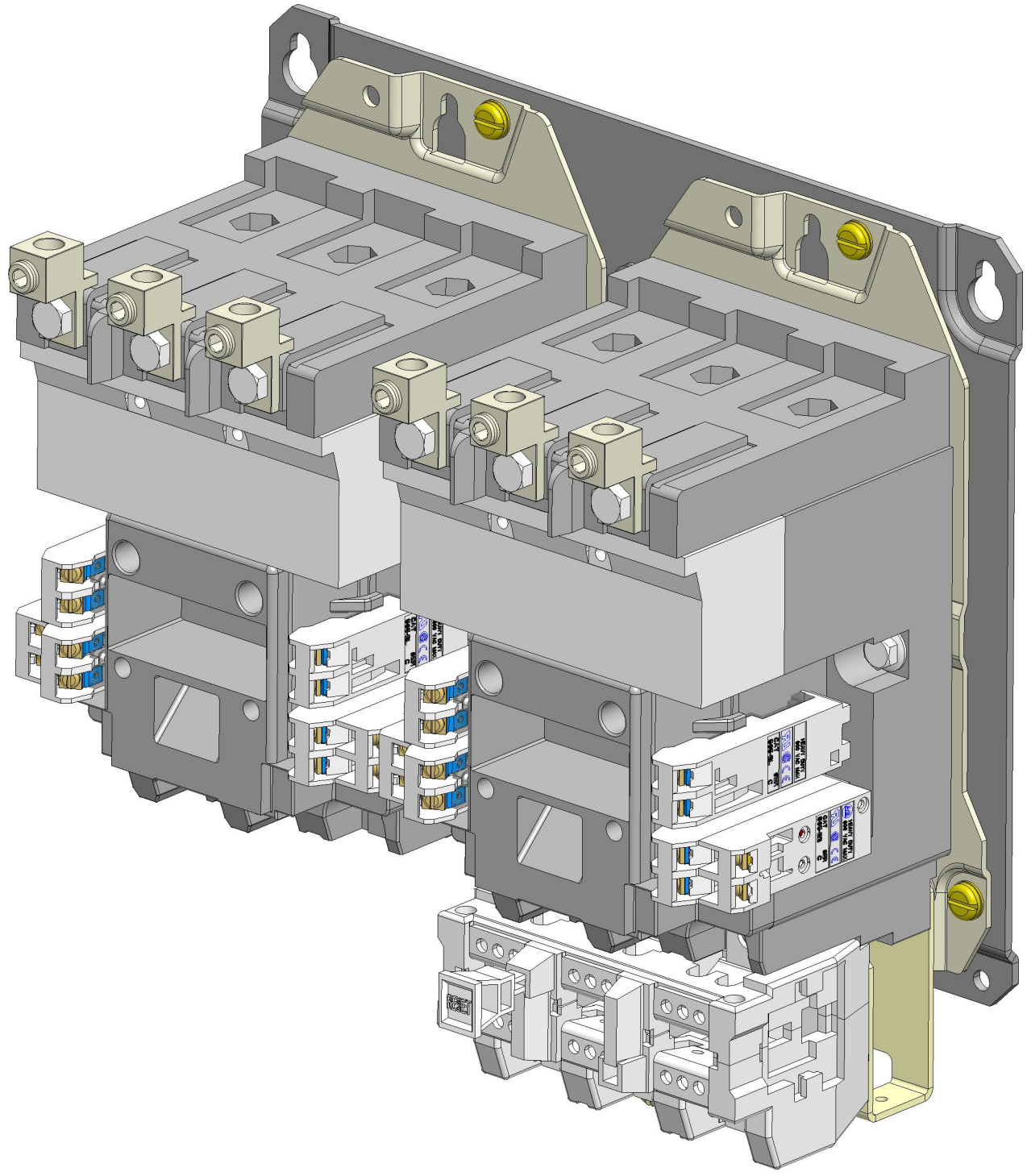
ISOMETRIC VIEW
