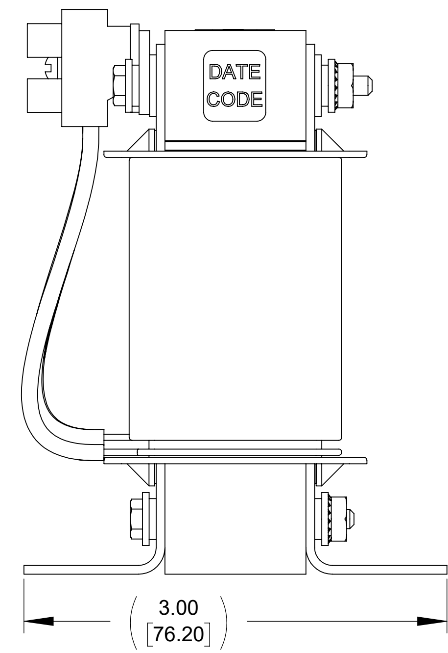
SIDE VIEW
