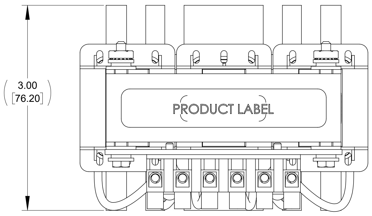
TOP VIEW
