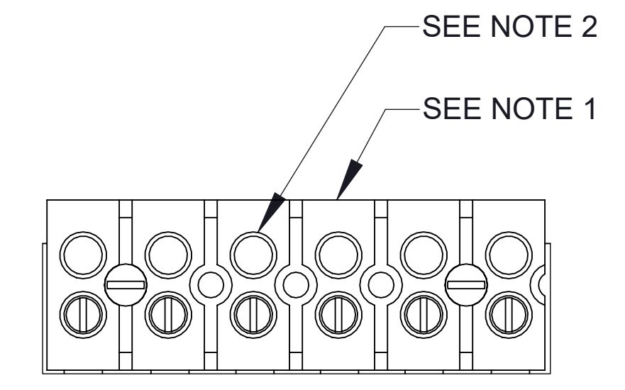
DETAIL A CUSTOMER CONNECTION DETAIL VIEW
