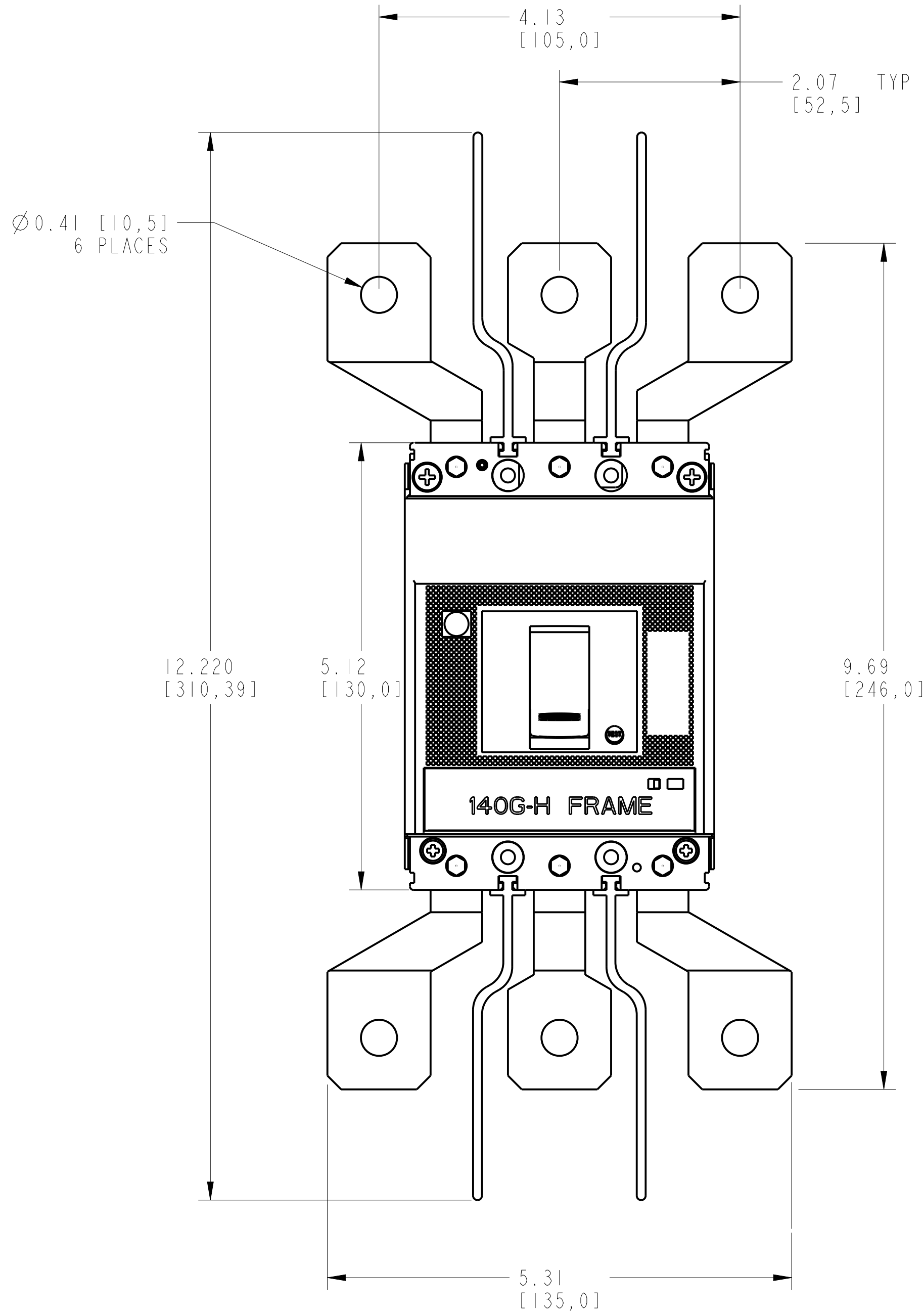
FRONT SPREADER TERMINAL ASSEMBLED TO 140G-H-3-POLE SCALE 0.9:1
