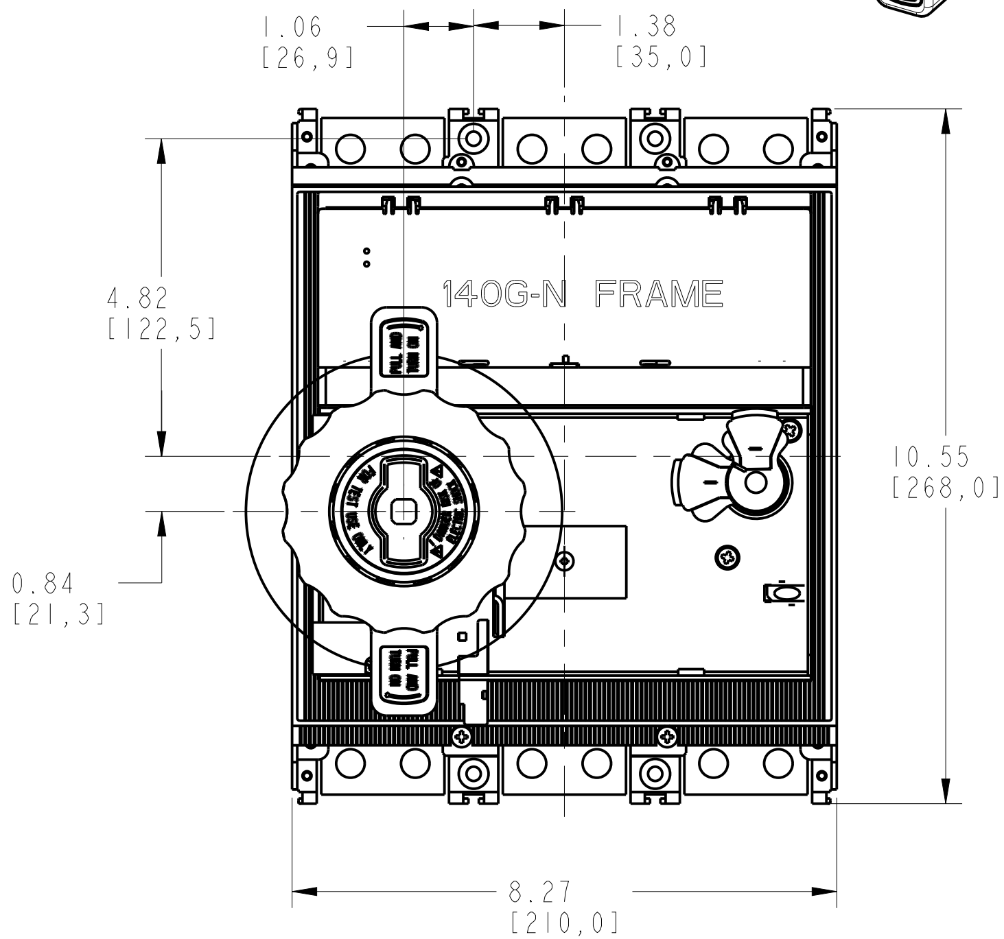
RHE SUPPORT ASSEMBLED TO 140G-N-3-POLE SCALE 0.5 : 1
