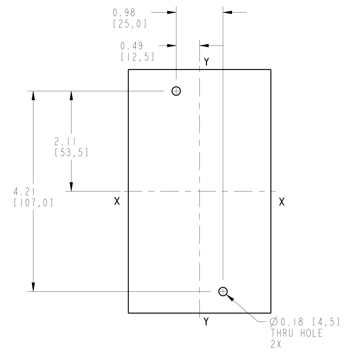
DRILLING FOR FIXING CIRCUIT BREAKER SCALE 1:1
