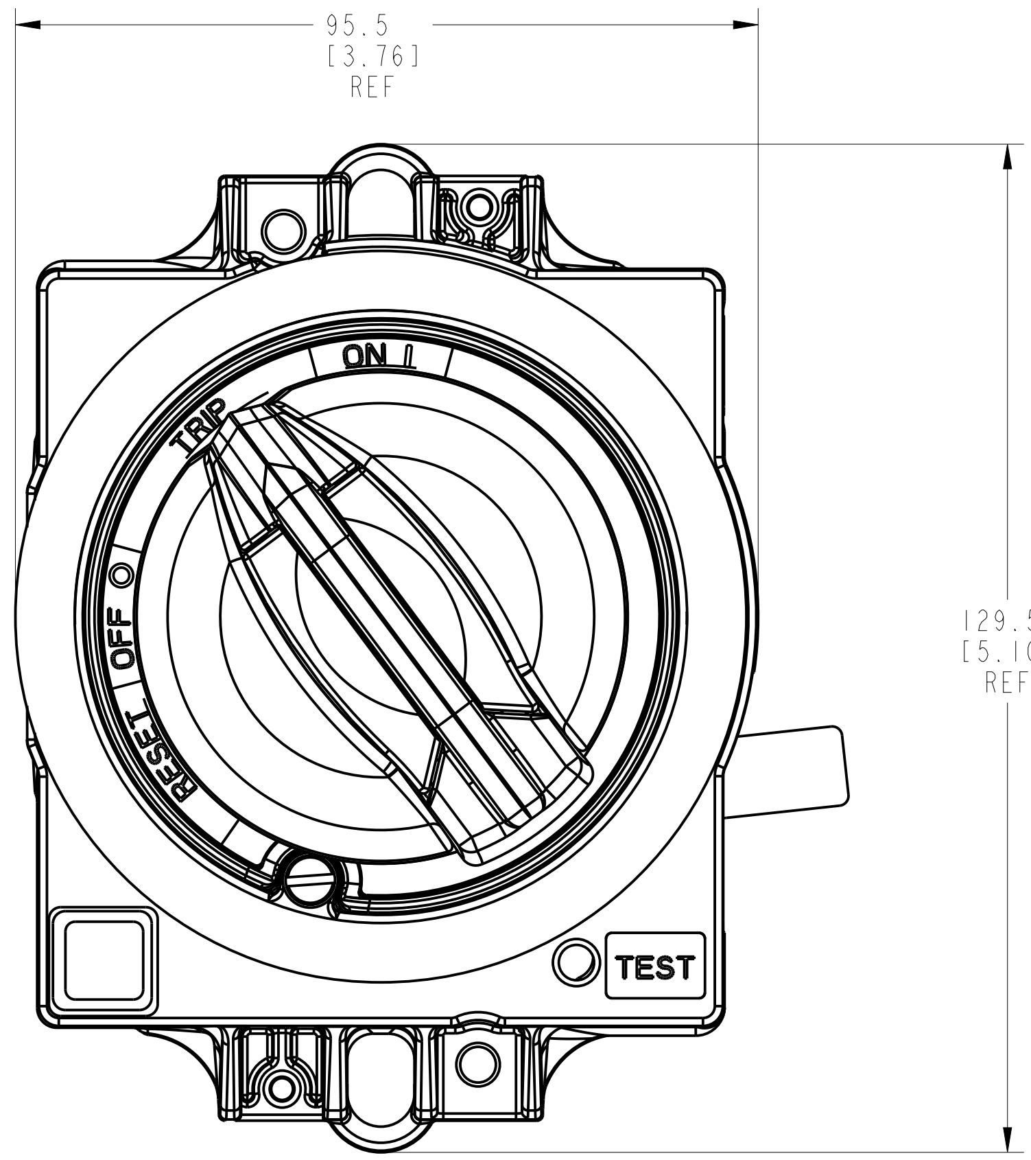
140G TTD G-FRAME DEPICTED
