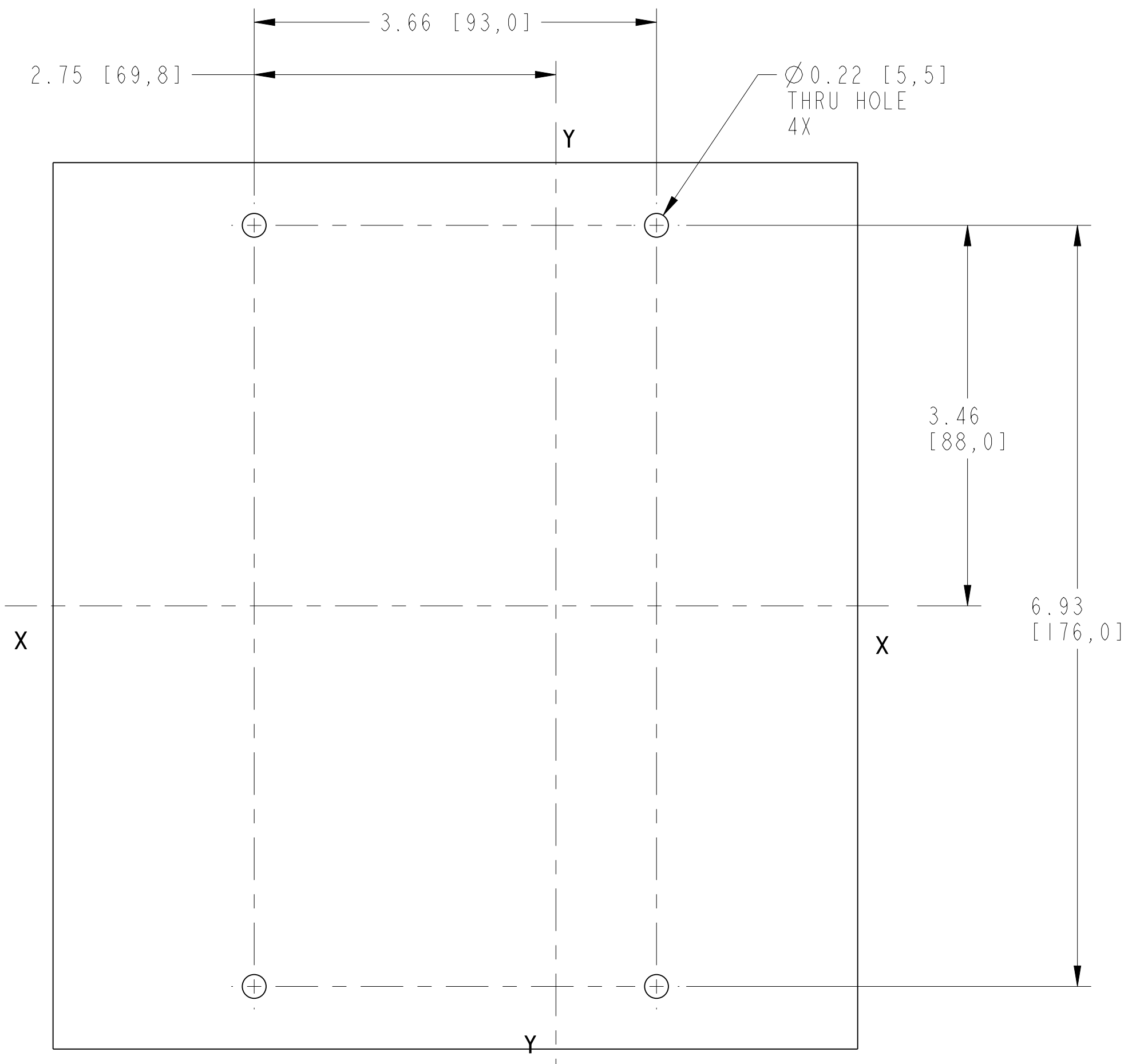
DRILLING FOR FIXING CIRCUIT BREAKER SCALE 1:1
