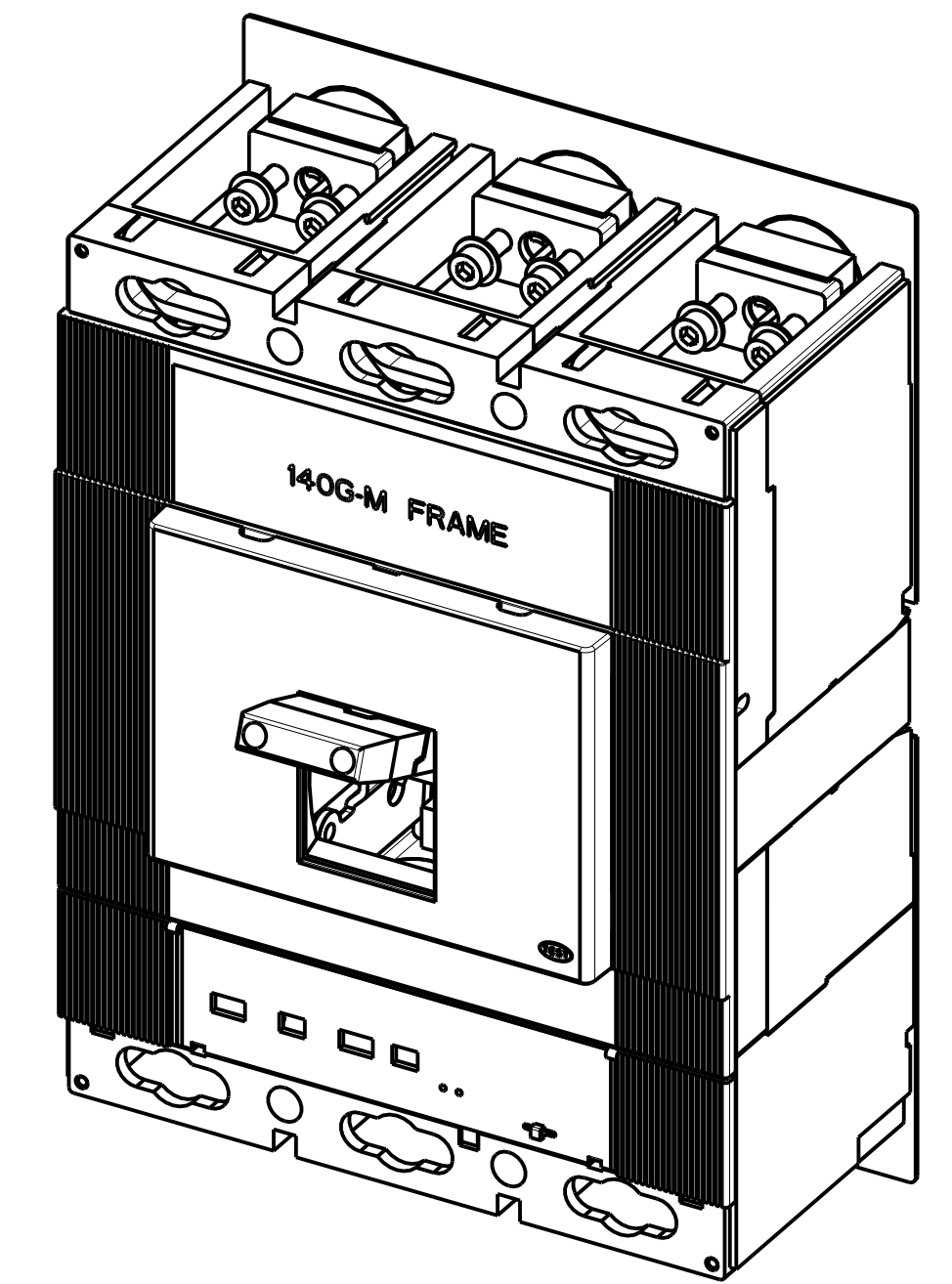
ISOMETRIC VIEW
