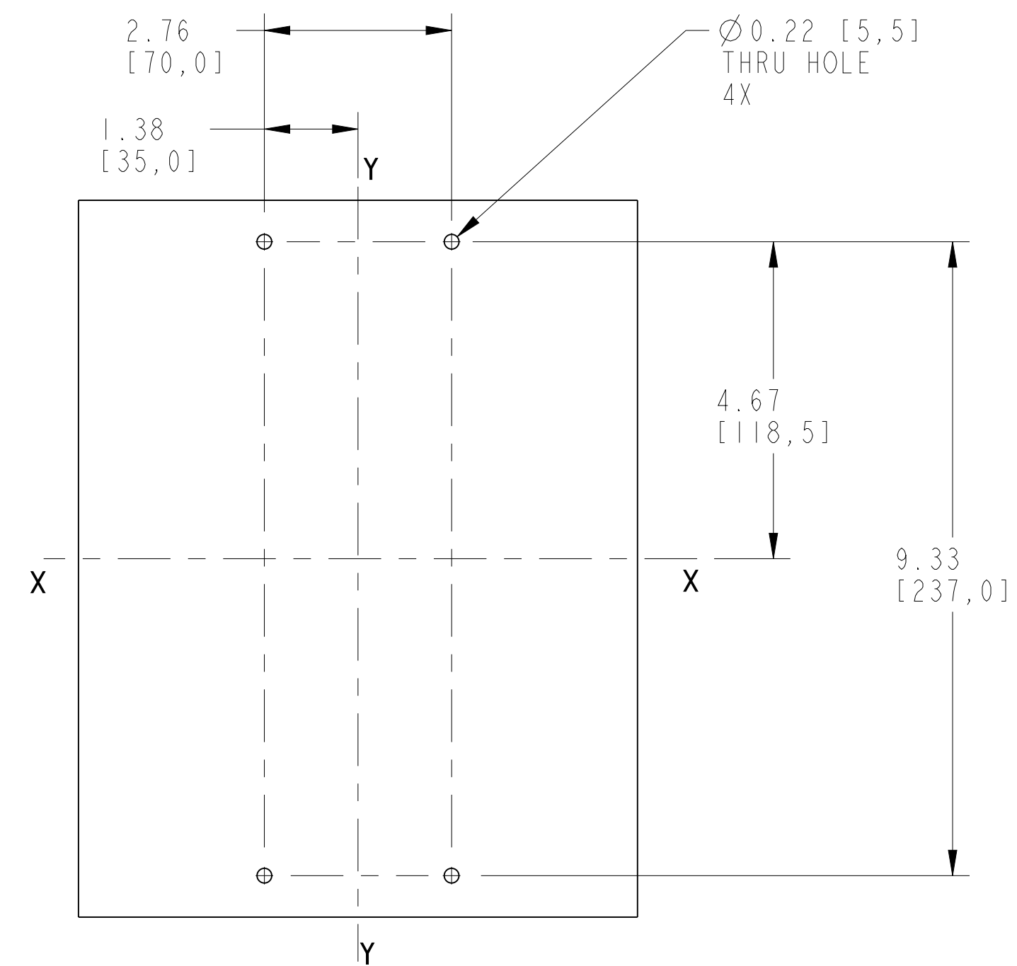
DRILLING FOR FIXING CIRCUIT BREAKER SCALE 0.5:1
