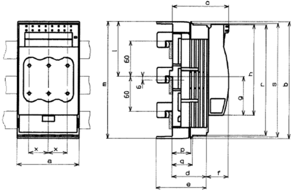
141A-NFJ30C, 141A-NFJ60C and 141A-NFJ100C
