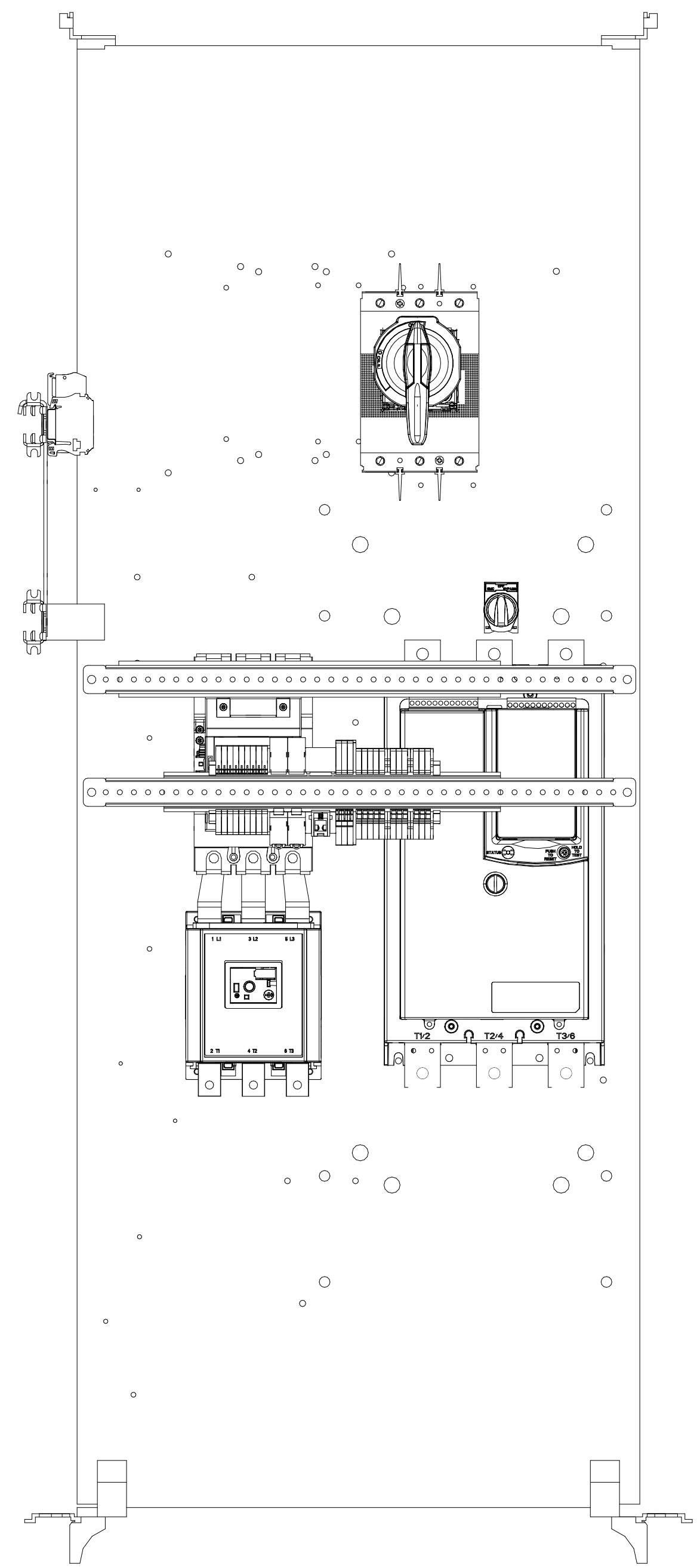
PANEL LAYOUT, (FRONT)
