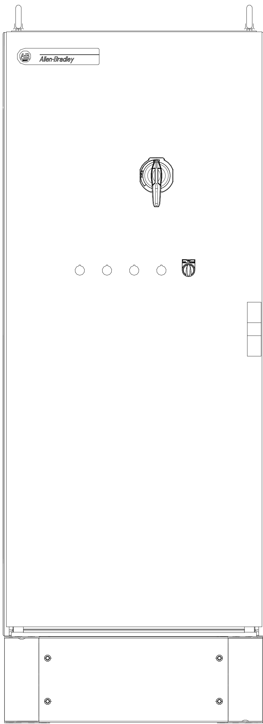
DOOR LAYOUT, (FRONT) ENCLOSURE SHOWN W/ DOOR, THIS VIEW
