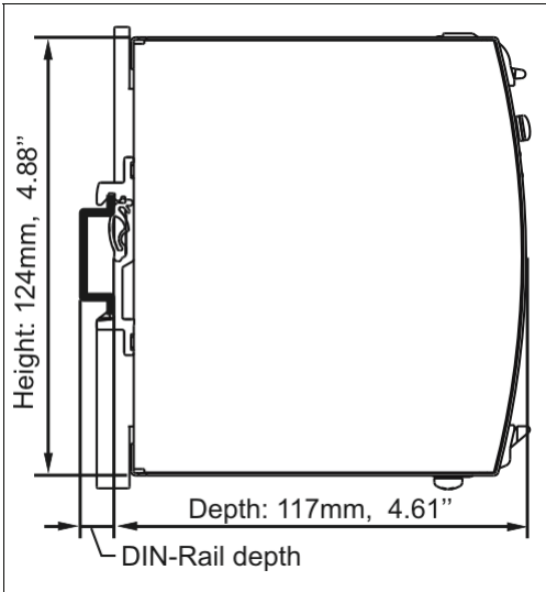
Fig. 22-2 Side view
