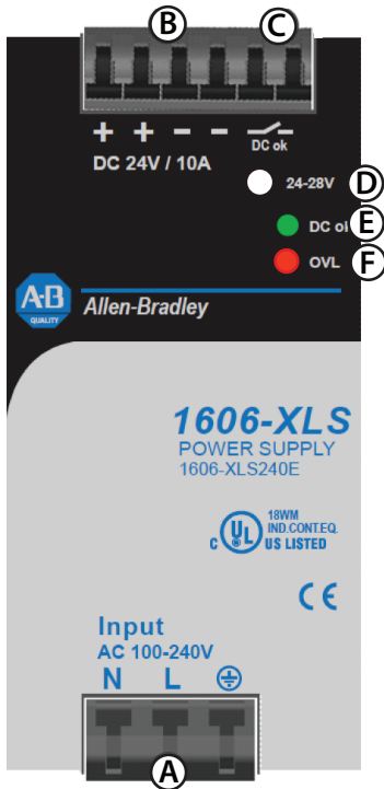
Fig. 13-1 Front side
