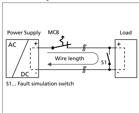
Fig. 23-5 Test circuit
