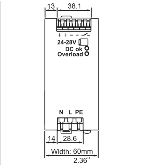
Fig. 22-1 Front view
