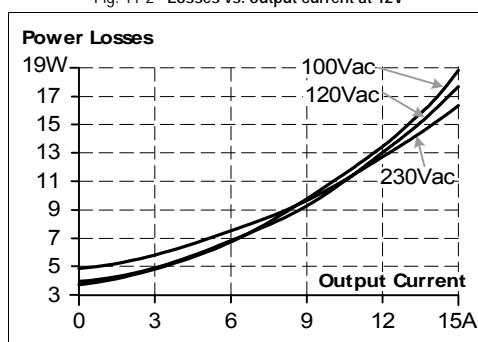
Fig. 11-2 Losses vs. output current at 12V
