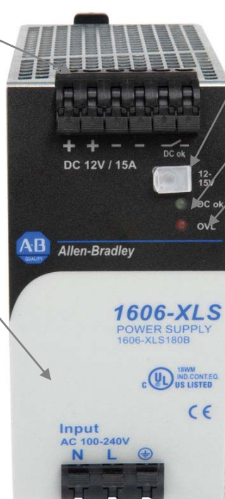
Fig. 13-1 Front side
