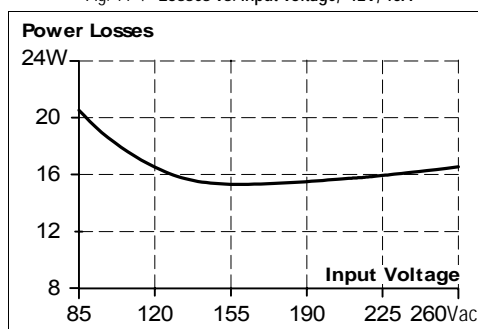
Fig. 11-4 Losses vs. input voltage, 12V, 15A
