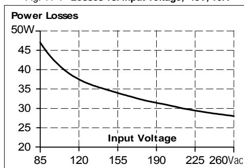
Fig. 11-4 Losses vs. input voltage, 48V, 10A
