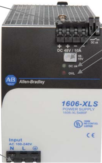
Fig. 13-1 Front side
