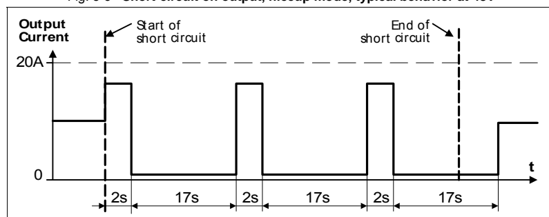
Fig. 8-3 Short-circuit on output, hiccup mode, typical behavior at 48V
