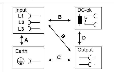
Fig. 20-1 Dielectric strength
