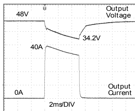
Peak load 80A (resistive) for 5ms Output voltage dips from 48V to 34.2V .
