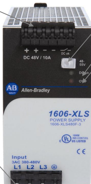
Fig. 13-1 Front side
