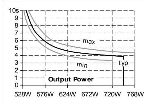
Fig. 8-2 Boost time vs. output power
