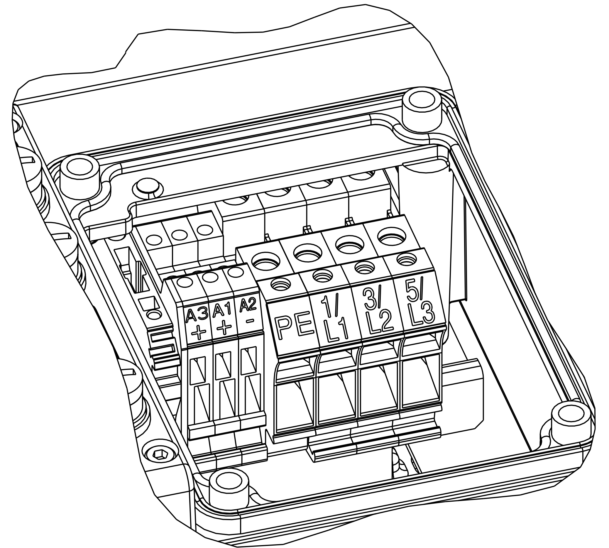
DETAIL A
