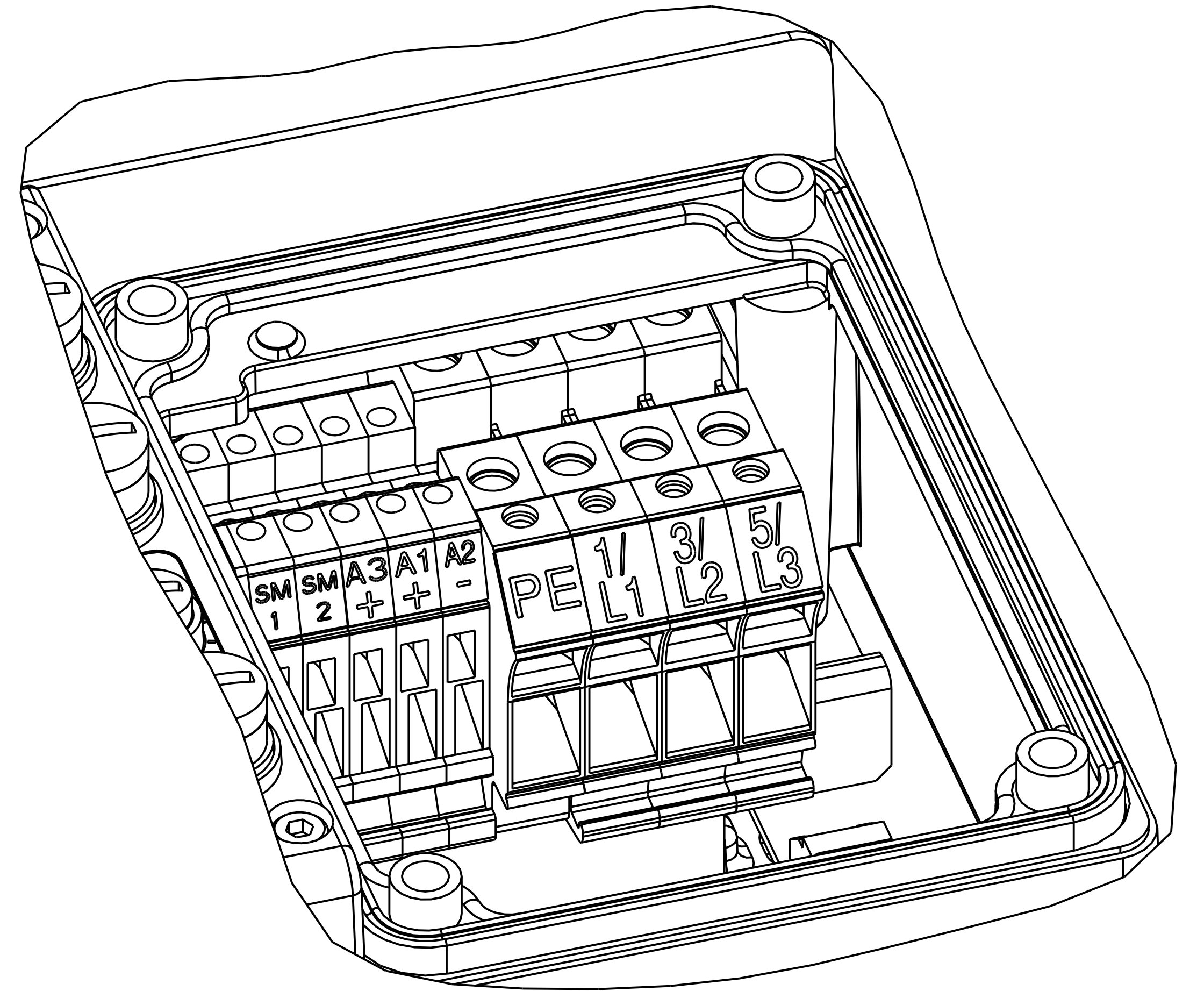
DETAIL A
