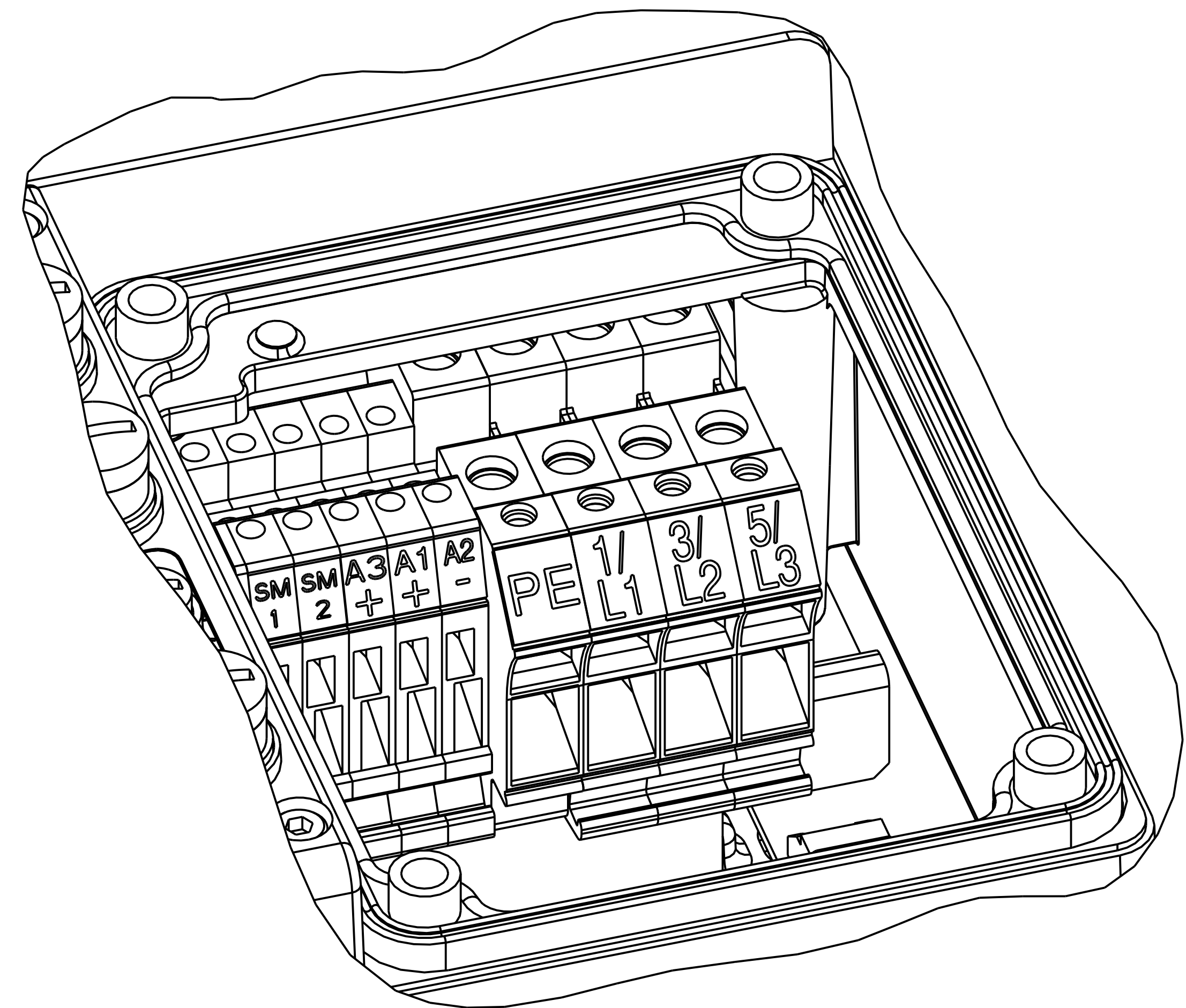
DETAIL A
