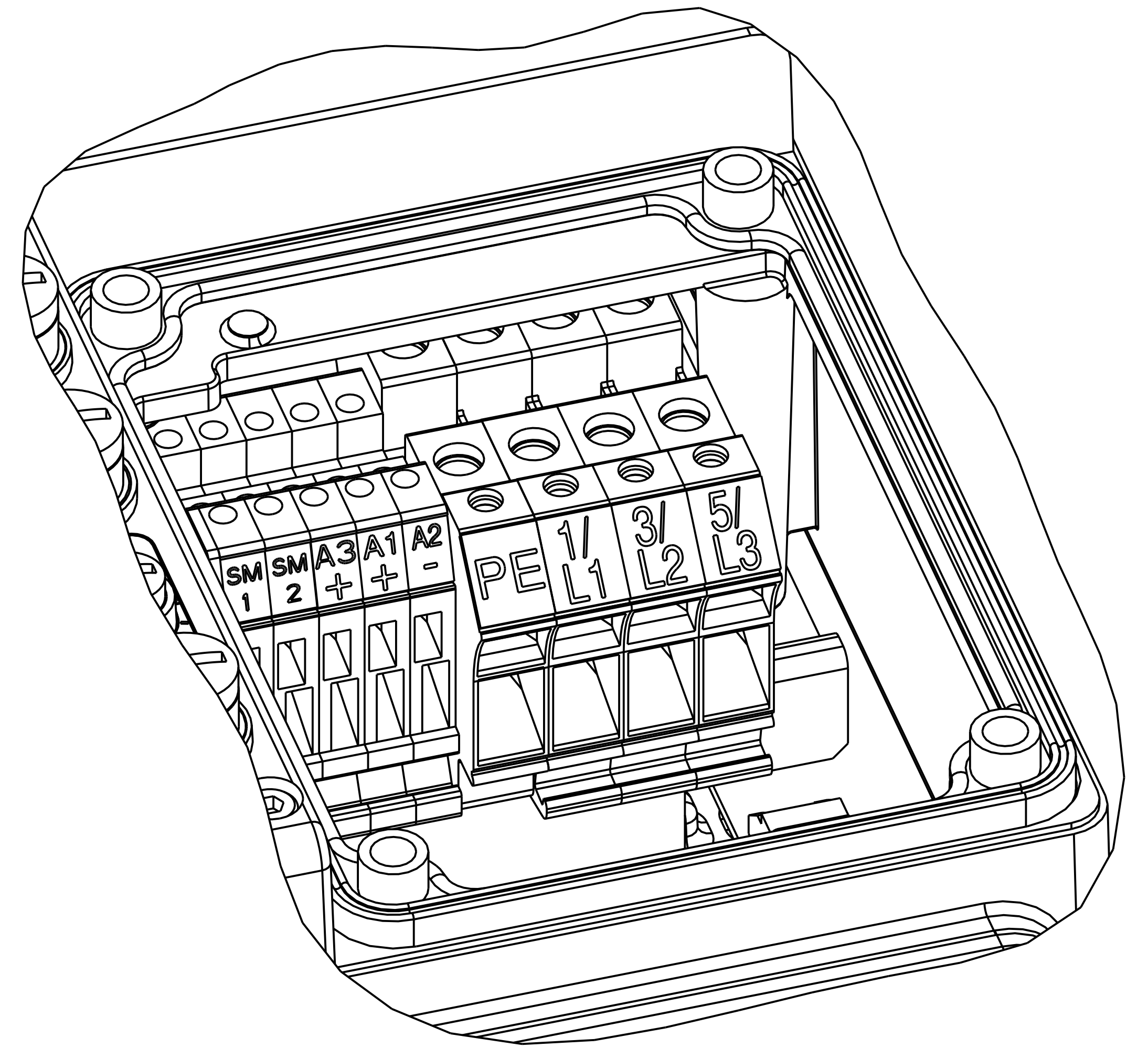
DETAIL A
