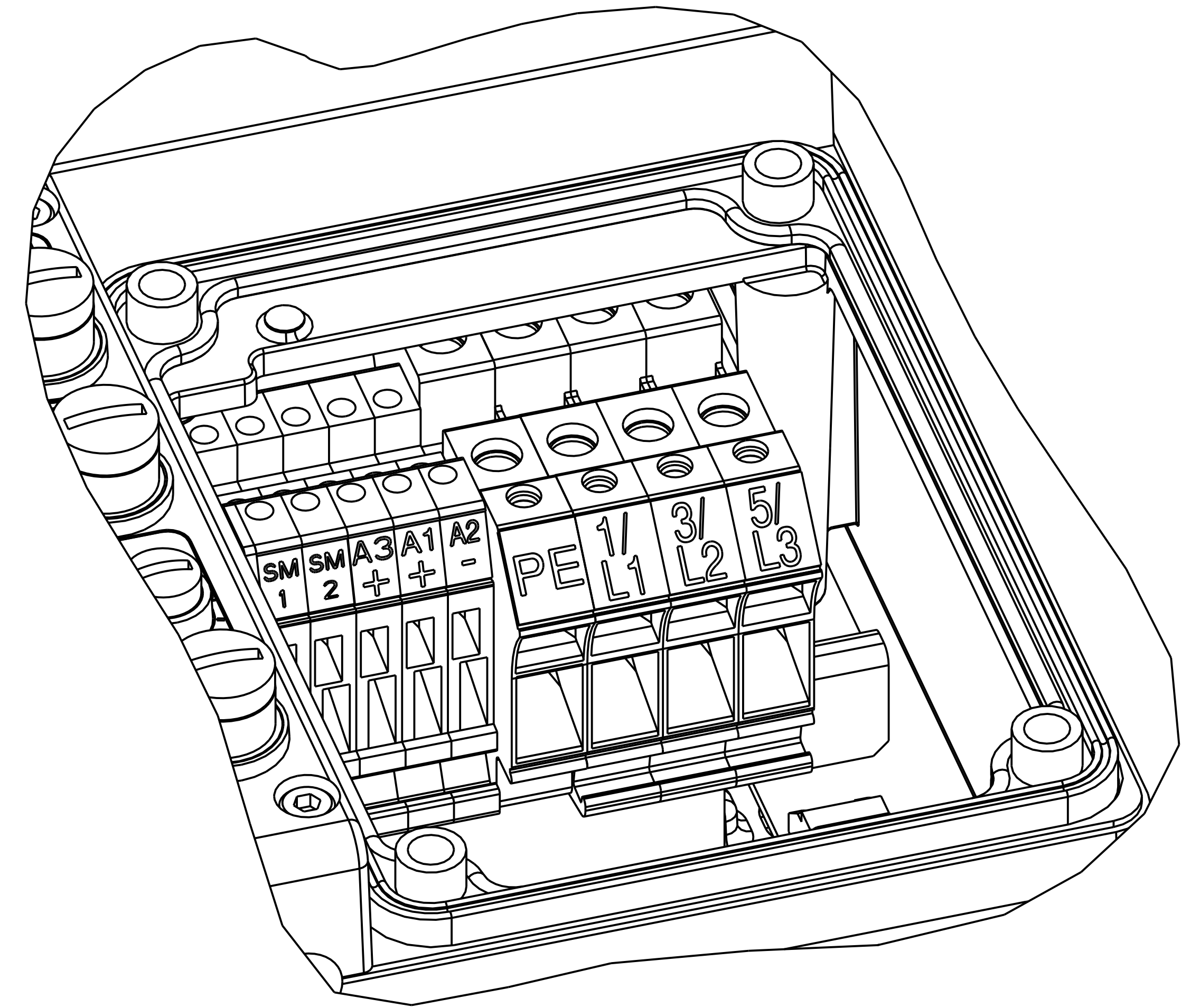
DETAIL A
