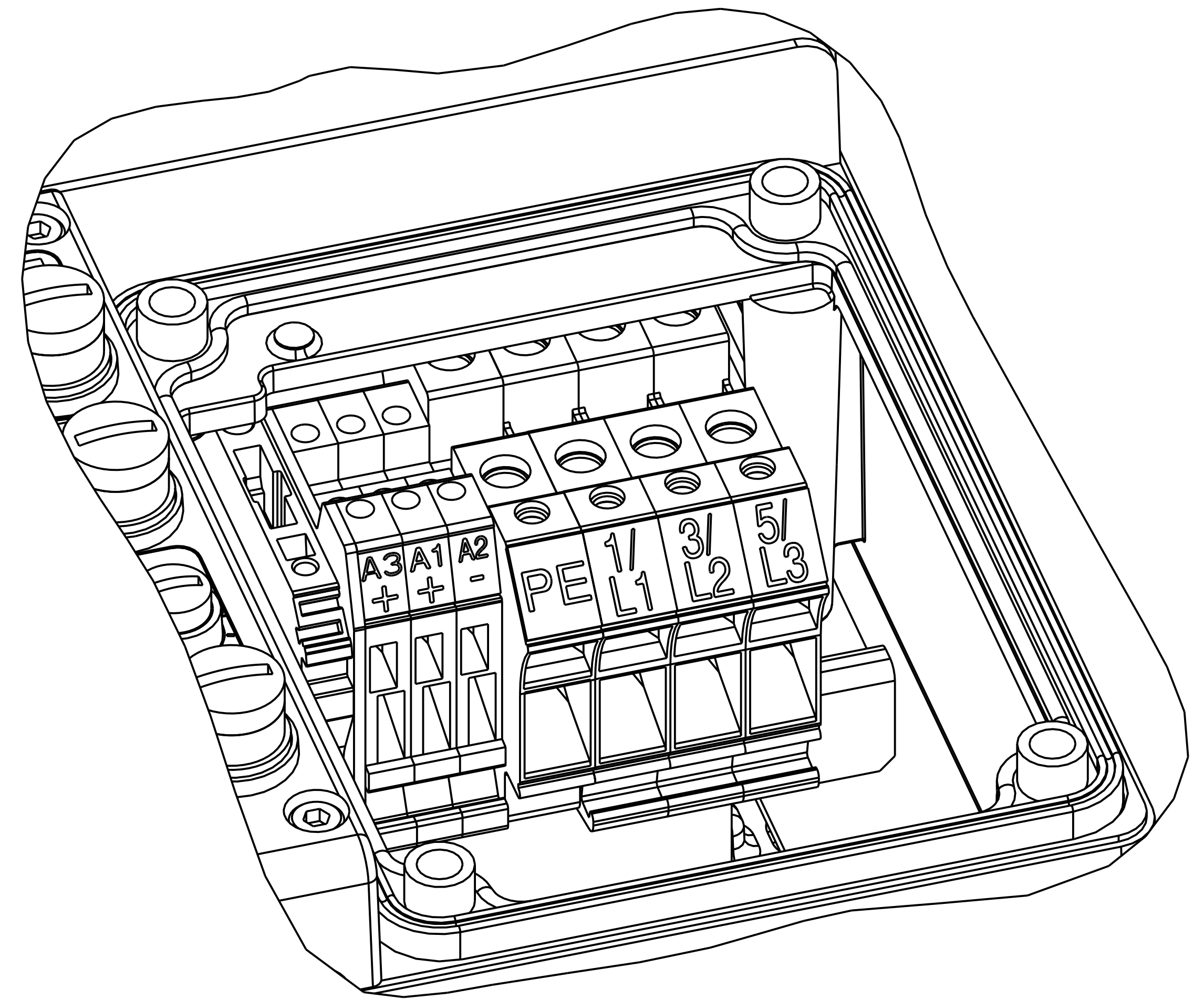
DETAIL A
