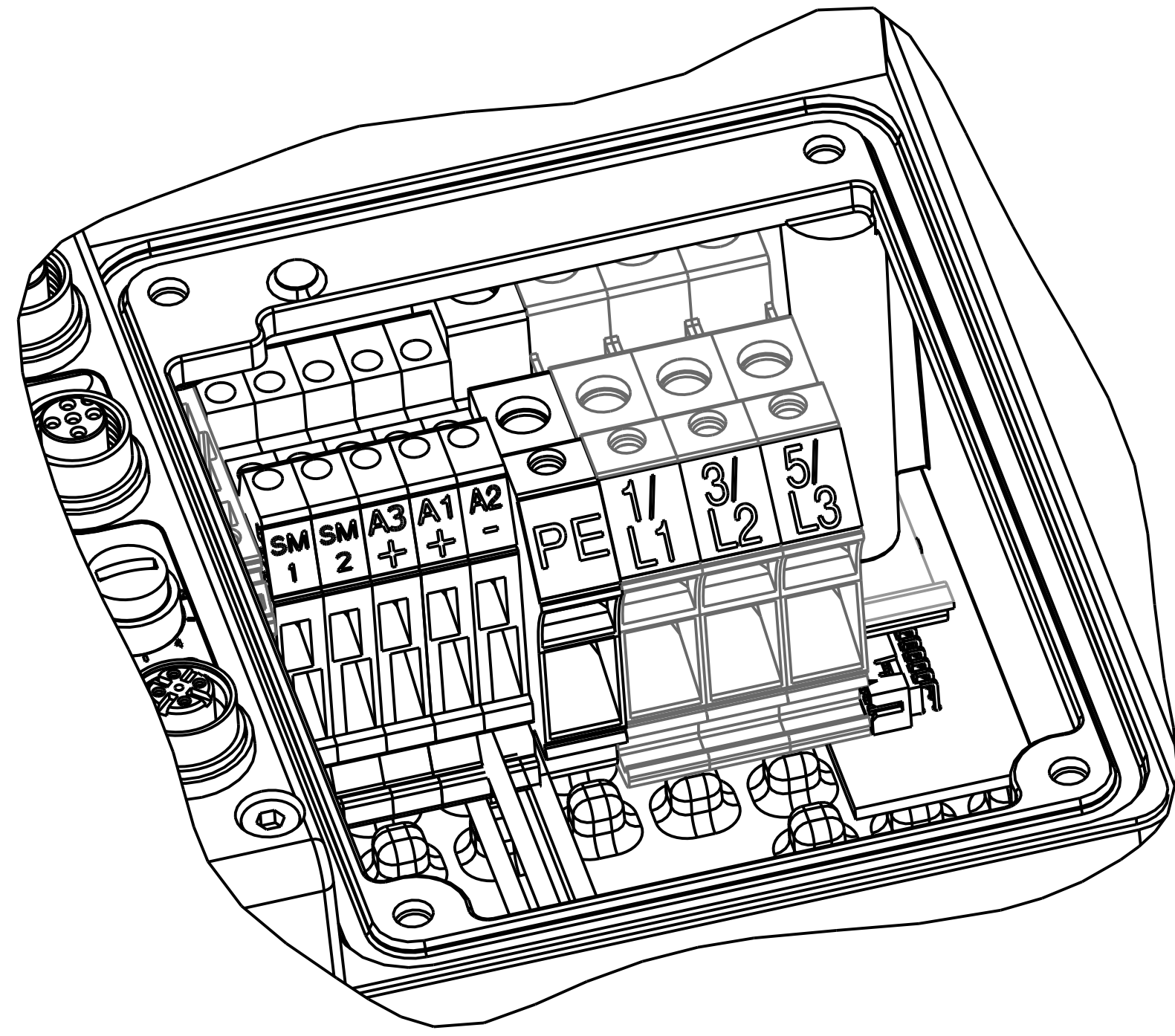
DETAIL A SCALE 1.500
