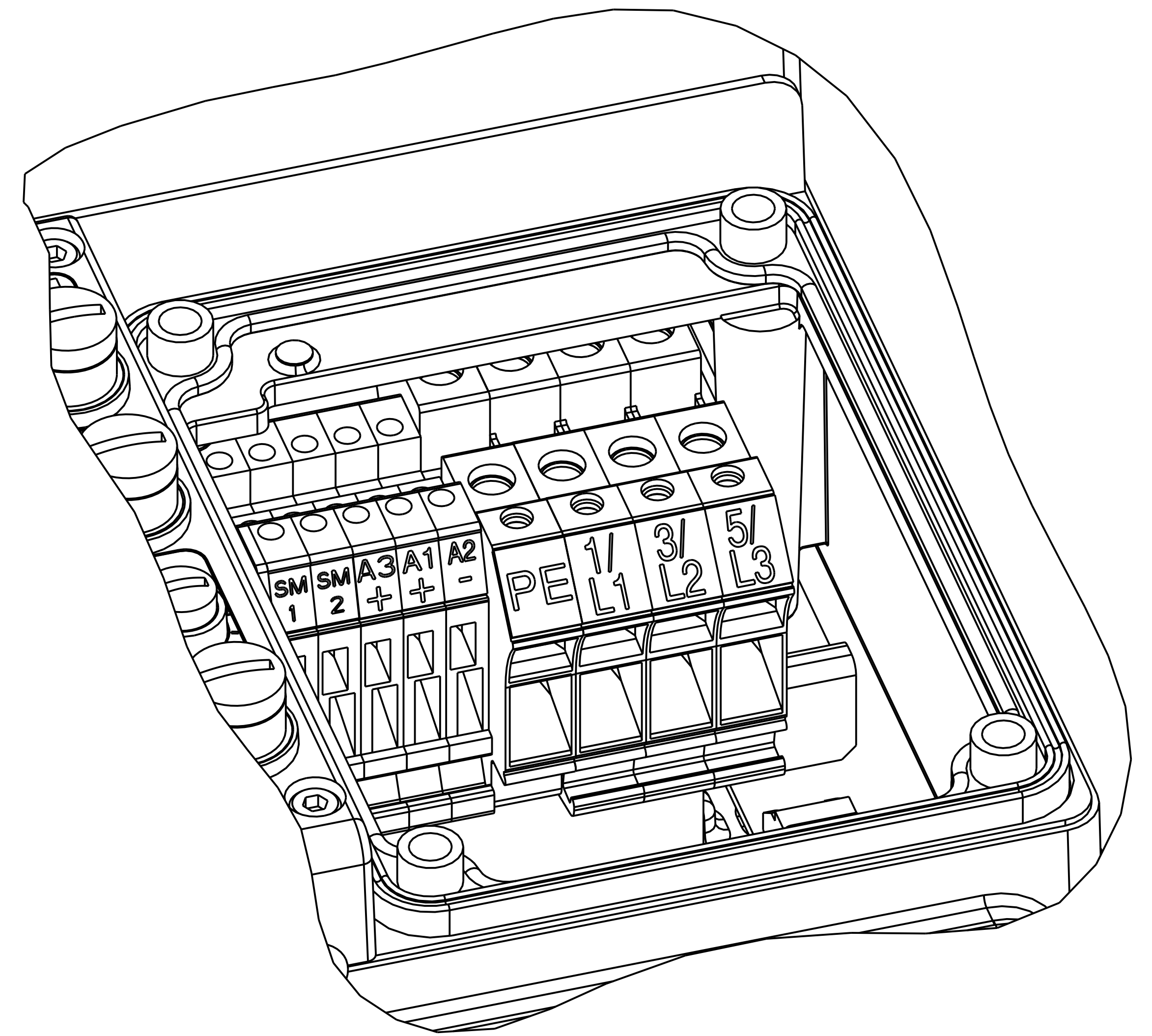
DETAIL A
