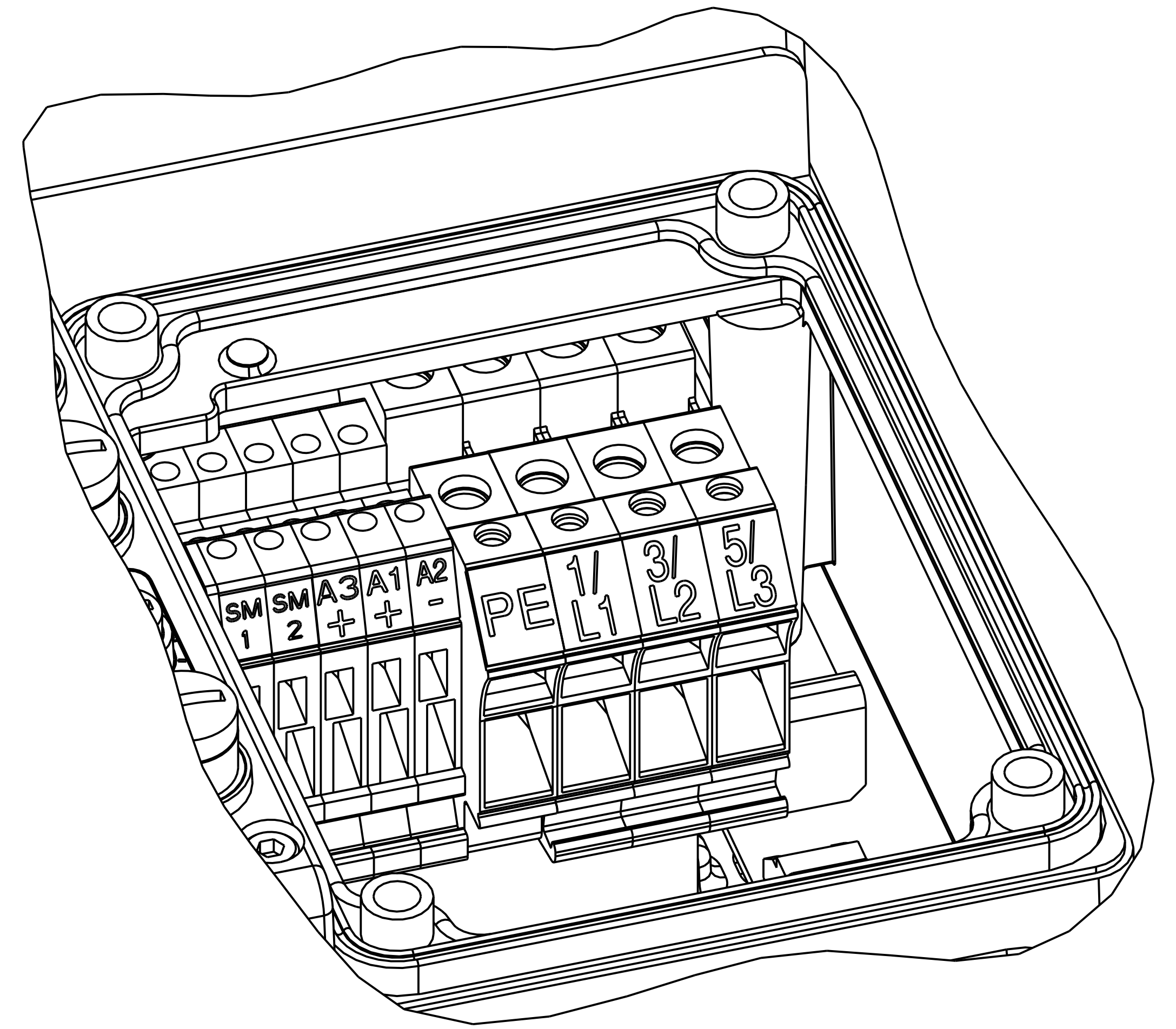
DETAIL A
