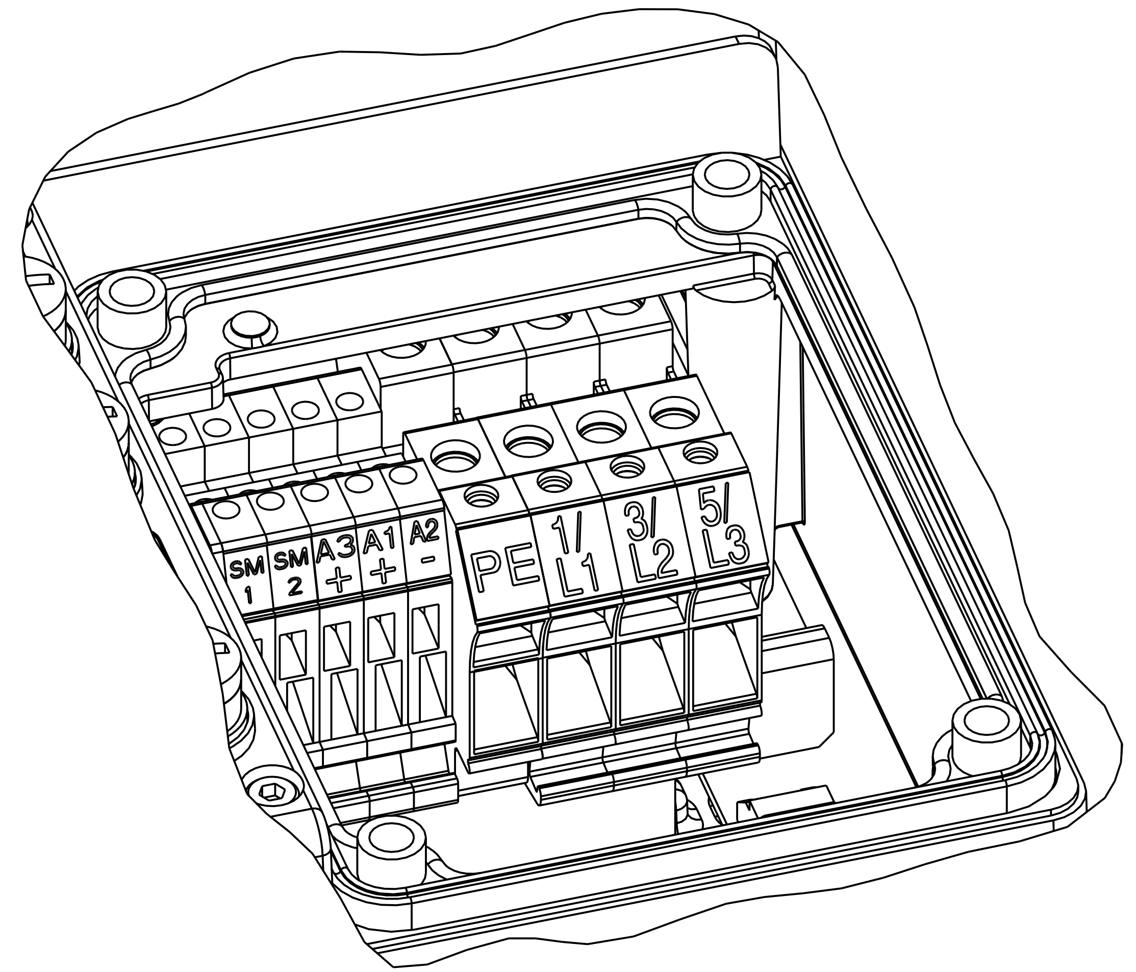
DETAIL A
