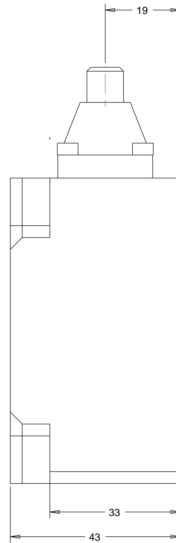
440P-METAL_DOME_PLUNGER
