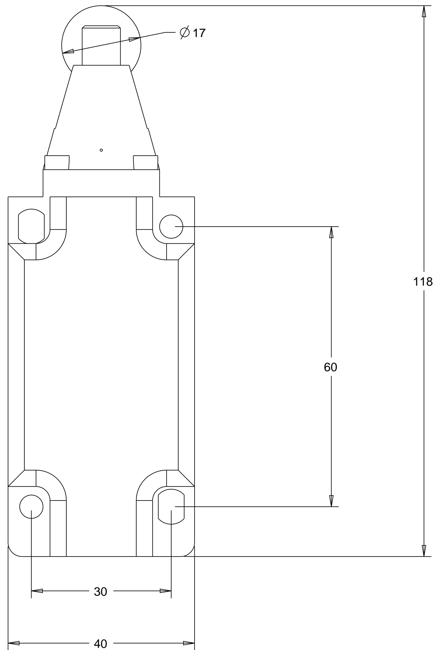
440P-ROLLER_PLUNGER
