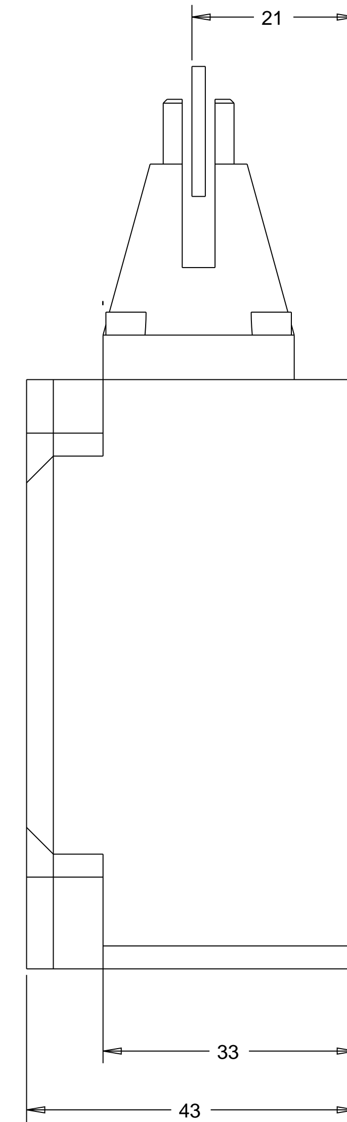
440P-ROLLER_PLUNGER
