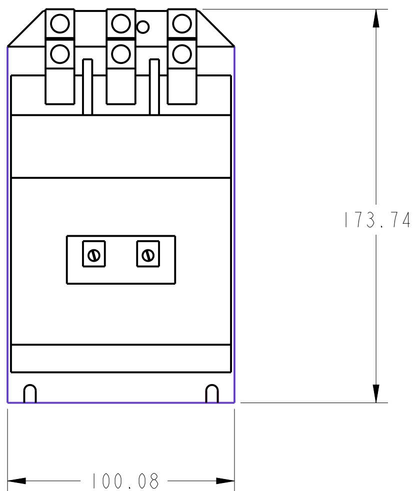
FRONT VIEW
