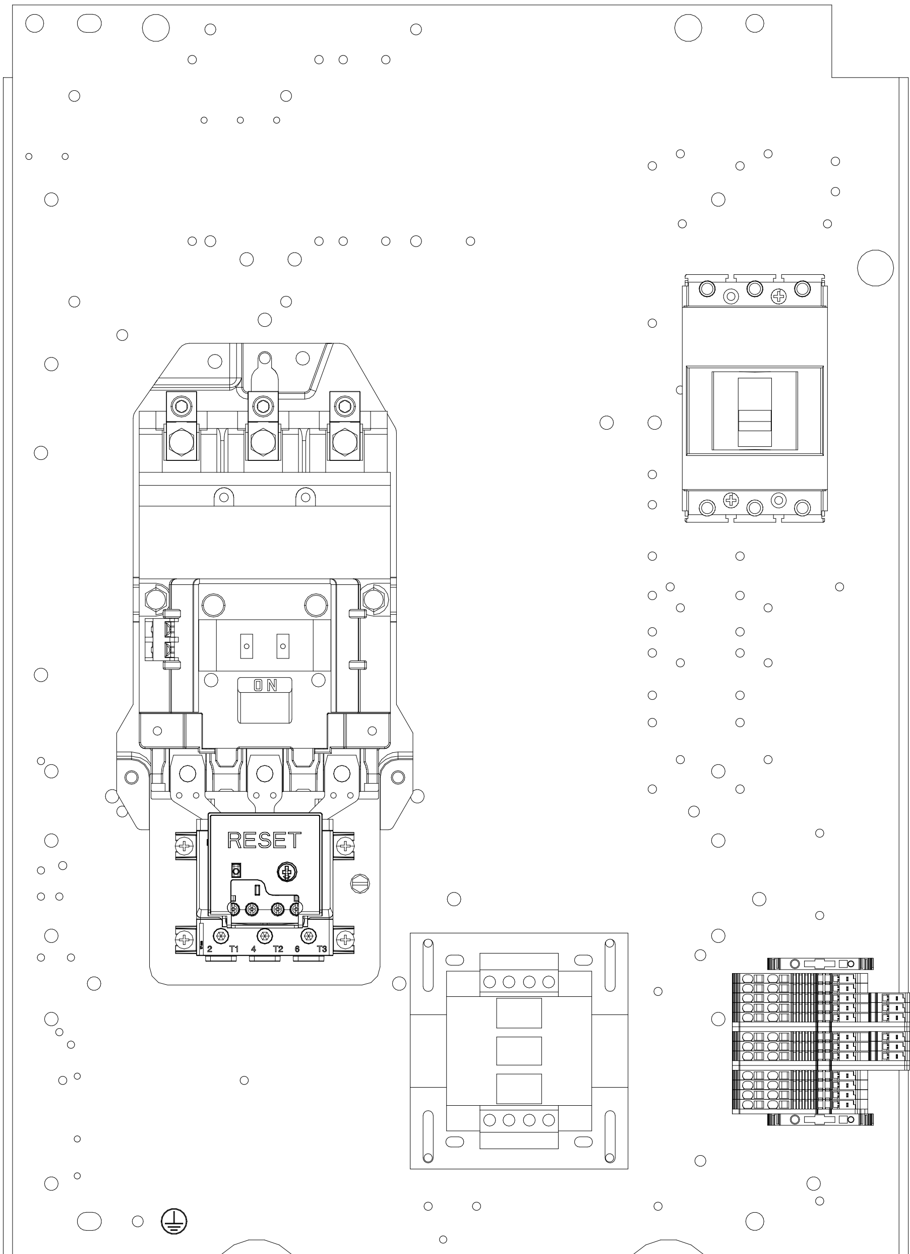
PANEL LAYOUT, (FRONT)
