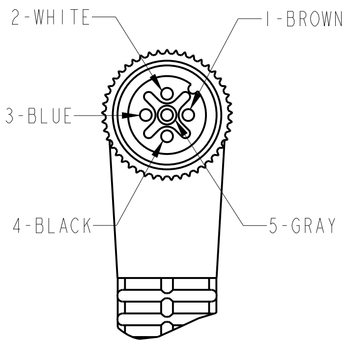
5-PIN, M12 RIGHT ANGLE MALE CONNECTOR
