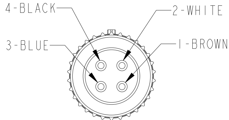
4-PIN, M8 X 1 STRAIGHT FEMALE CONNECTOR
