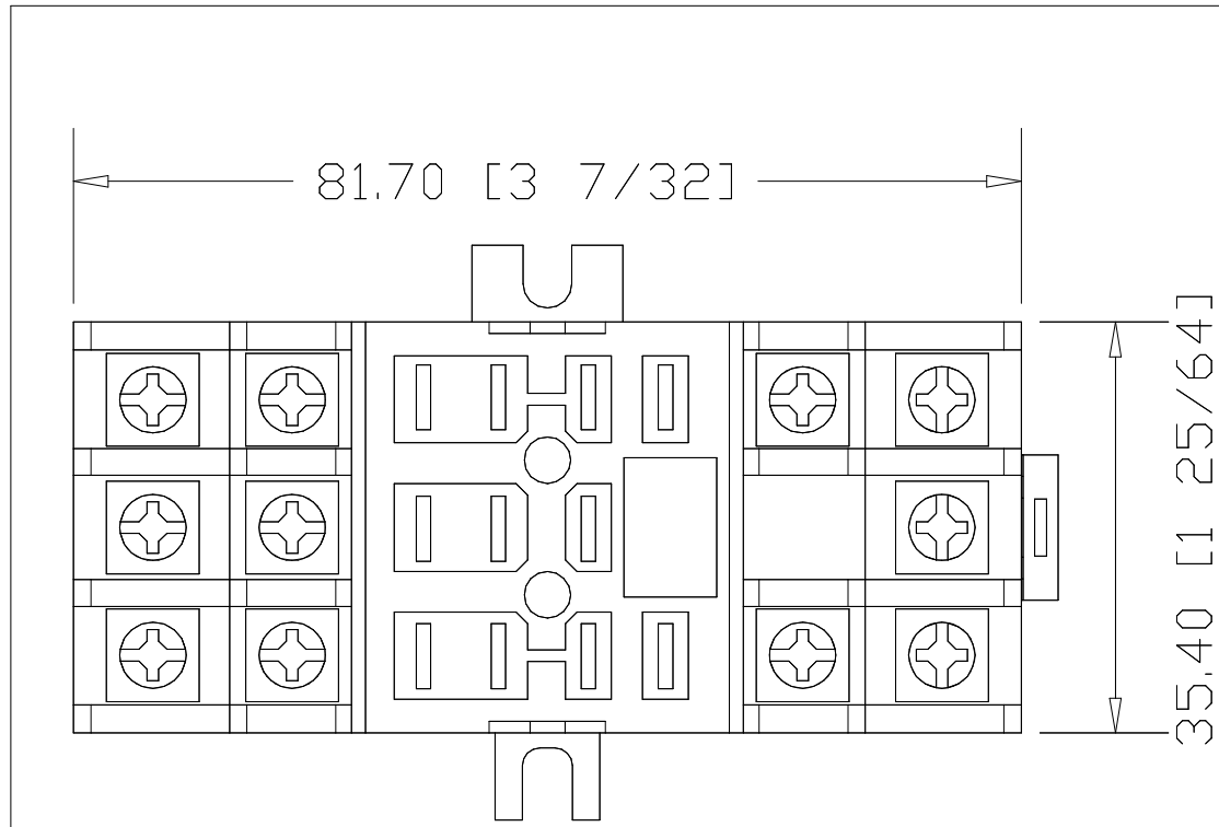
700-HN154 Socket, Open Terminal
