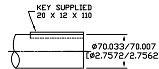
DRIVE END SHAFT DETAIL SPEC (9)
