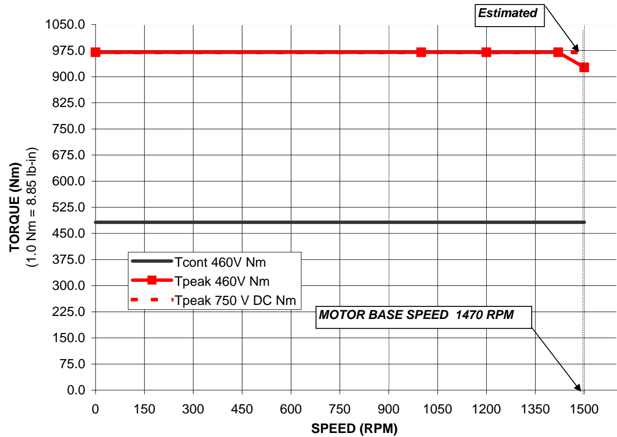
HPA-B2010C-MA42AA Performance with 2099-BM11 at 460 VAC and 750 V DC Drive Input, 40C Motor Ambient
