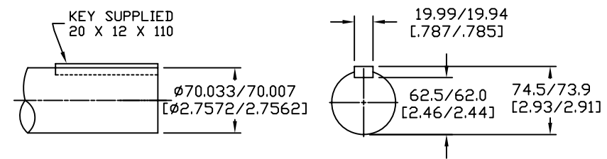
DRIVE END SHAFT DETAIL SPEC (9)
