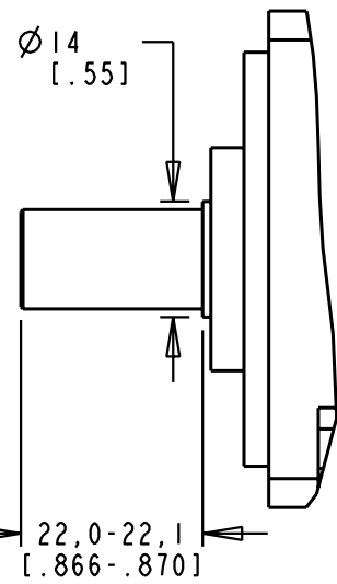
SHAFT DETAIL (NO SCALE)
