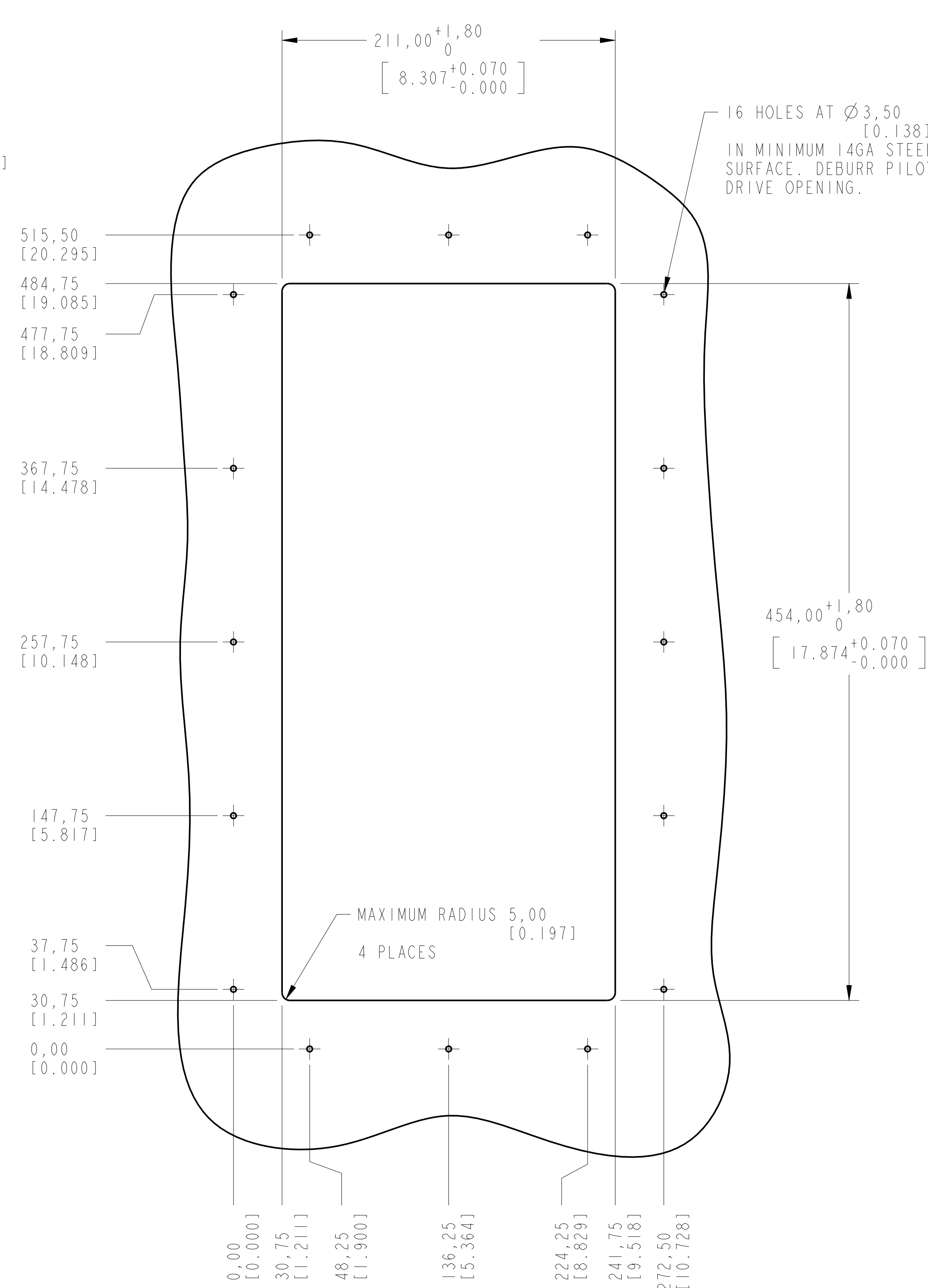
TYPE 4X, FLANGE MOUNT
