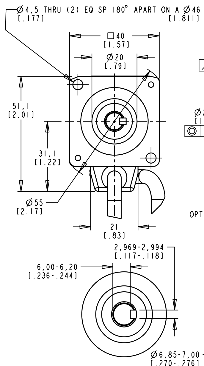
SHAFT DETAIL (NO SCALE)
