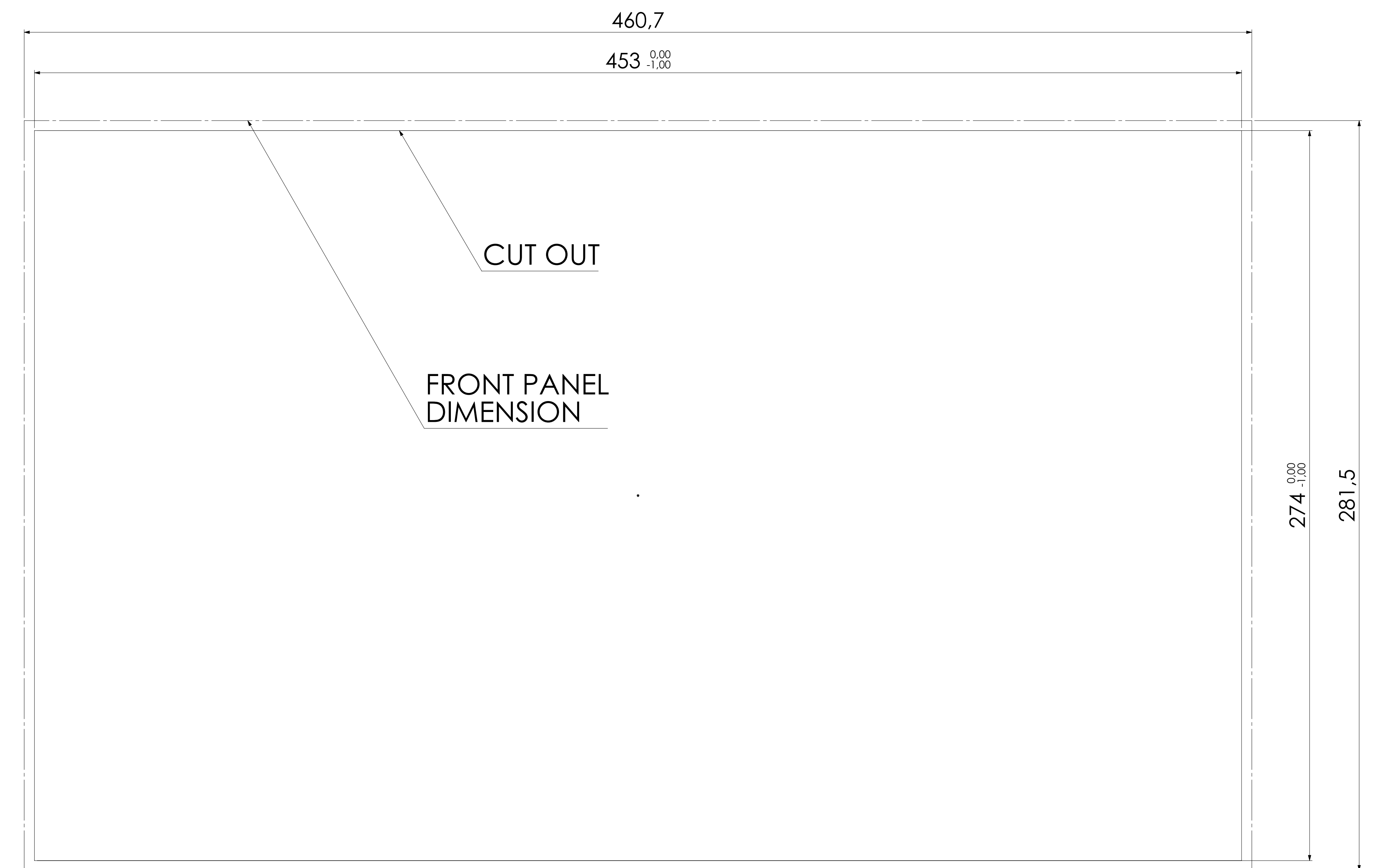
VersaView 6300P (Fanless) 6300P-185ECPMFDNA 18.5 Inch Display dimensions are in mm
